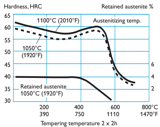
TEMPERING GRAPH
